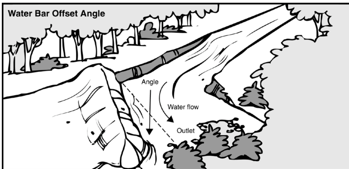
Diagram 9.3.5.4b – Water bar offset angle
