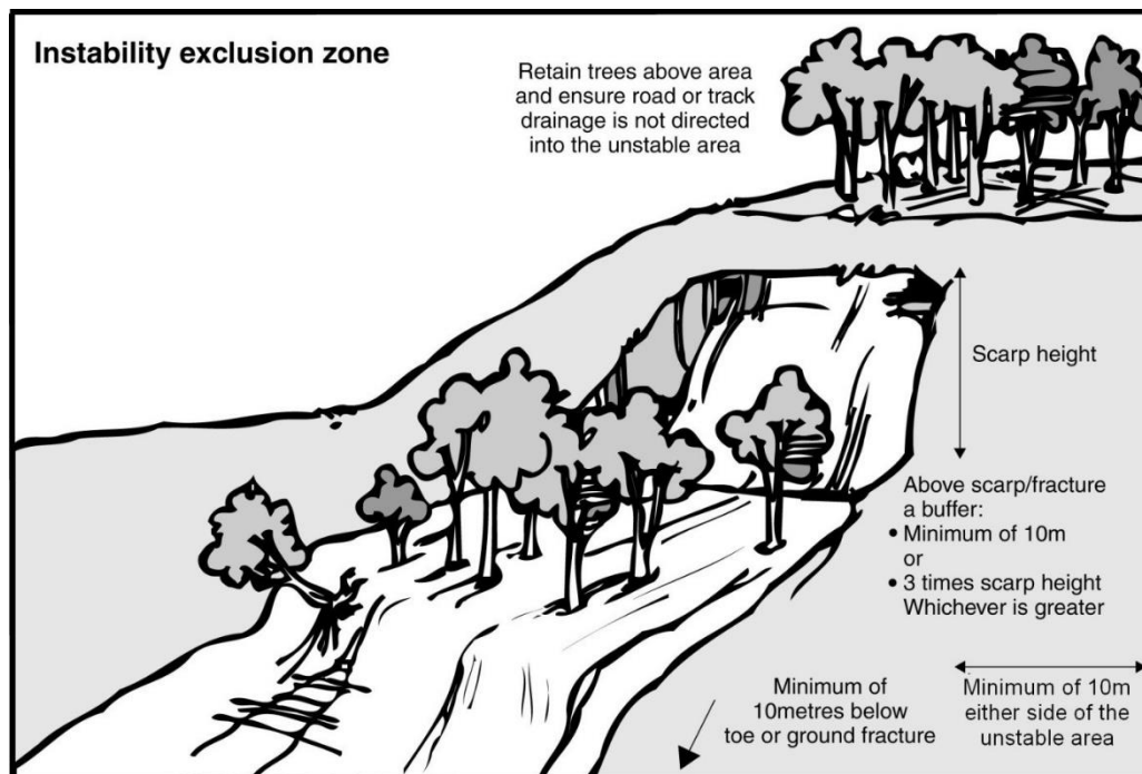
Diagram 5.2 – Instability exclusion zone
