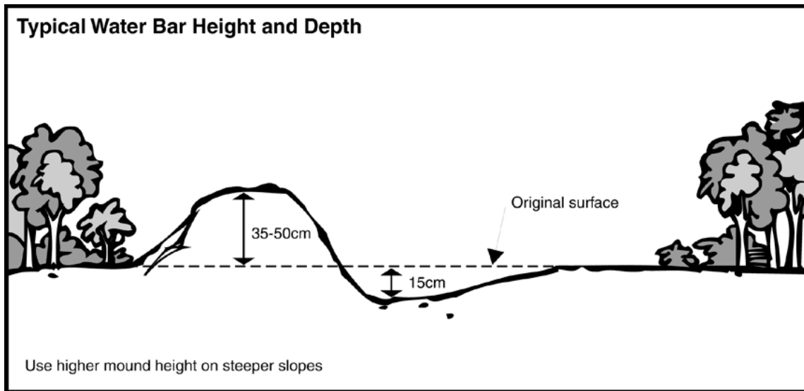
Diagram 9.3.5.4c – Example of a typical water bar height and depth
