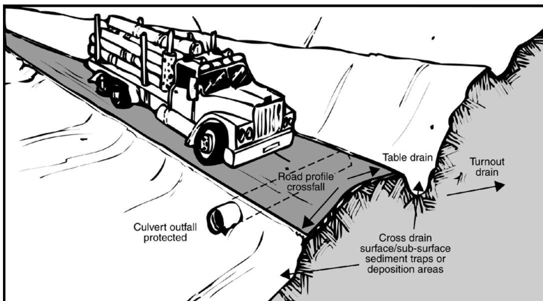
Diagram 9.1 – The basic road drainage system for A, B and C type formations.
