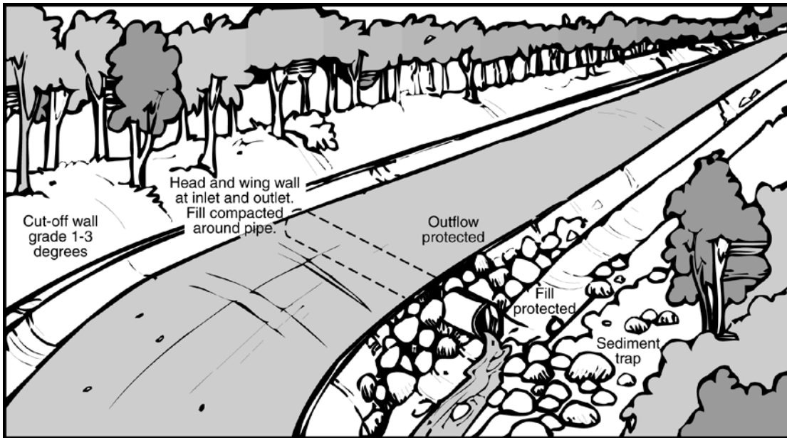
Diagram 9.3.5.1 – Typical pipe culvert
