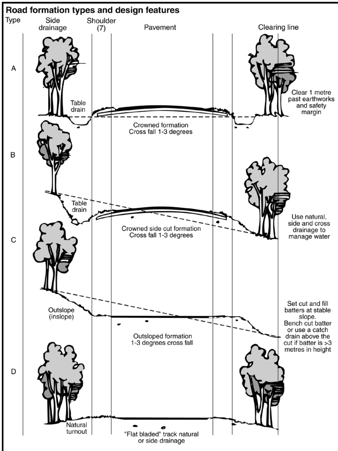
Diagram 8.4 – Road formation types and design features
